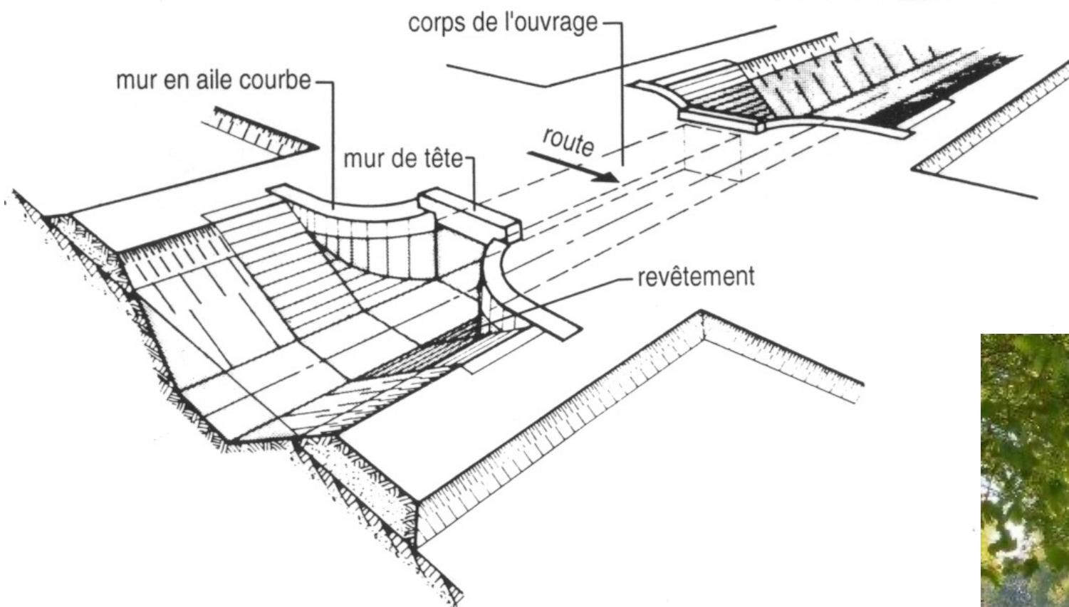
Dalot with progressive connection
